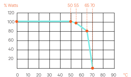
Figure 3: Output Power vs. Temperature at 264 VAC \geq V_{in} \geq 176 VAC and 58 VDC \geq V_{out} \geq 48 VDC
