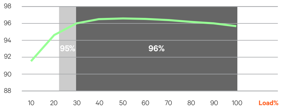
Rectifier Efficiency Curve at 220 VAC Nominal
