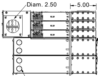
Left Side View Diam. 1.1 (4-places)
