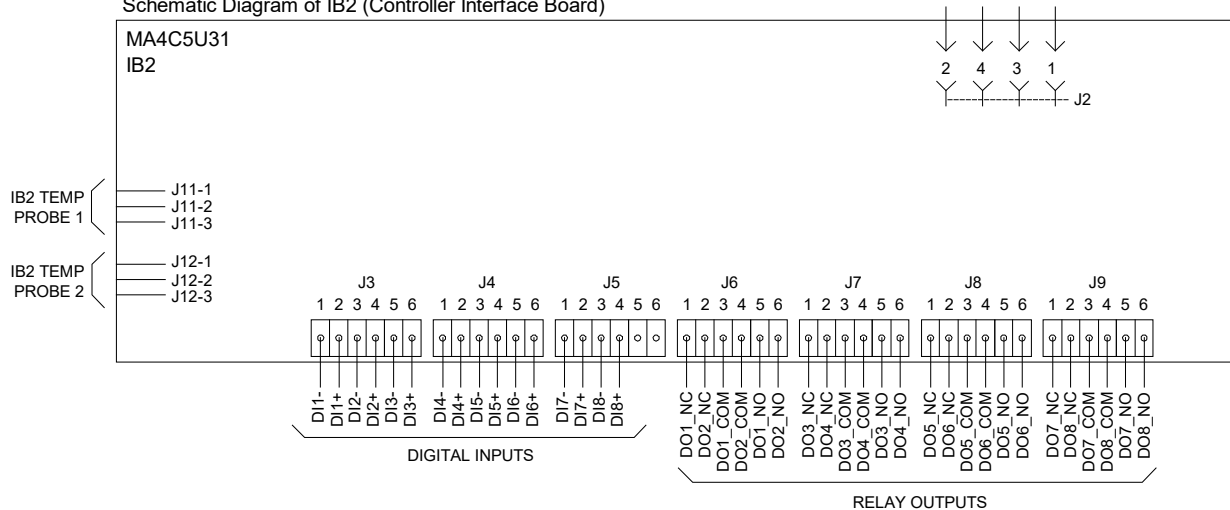
Figure 7 IB2 (Controller Interface Board)
